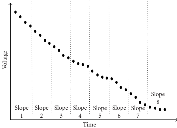
FIGURE 4: Least squares fitting of sub-ramps for 32-sample ramp over every 4 samples of a ramp.
