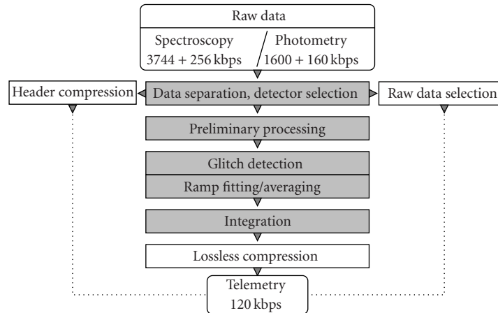
FIGURE 3: A schematic diagram for on-board processing concept. (Dark grey color indicates the modules where raw data are lossy compressed.)
